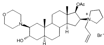
Figure 1. Chemical structure of rocuronium bromide, the target guest molecule of this study.
