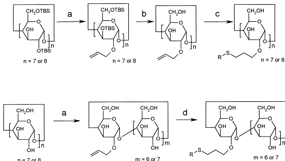
Scheme 2. Synthesis of 2- O alkylated CDs; (a) Allyl iodide, NaH. o/n; (b) TBAF, 1 h; (c) RSH, AIBN \Delta 2–24 h (d) RSH, AIBN, 1 h, \Delta . Toluene, MeCN water or MeOH. 100% conversion.
