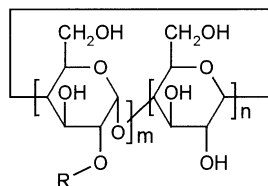
Figure 2. General formula of the modified CDs reported in this paper. For per-substituted \gamma -CDs m=8 , n=0 ; for mono-substituted \gamma -CDs m=1 , n=7 . For per-substituted \beta -CDs m=7 , n=0 ; for mono-substituted \beta -CDs m=1 , n=6 . R = alkyl or substituted benzyl groups.
