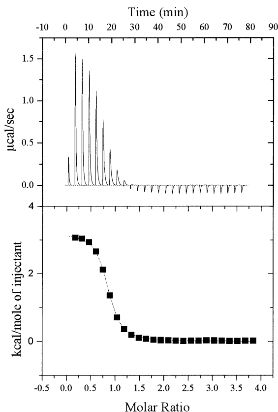
Figure 3. Isothermal titration calorimetry of compound 1 and rocuronium bromide. A buffer solution (pH 7.0) of rocuronium bromide (1.5 mM) was titrated into the same buffer solution of compound 1 (0.075 mM). The results show the endothermic complexation between 1 and rocuronium, \Delta H = 3198 \pm 12.06 \text{ cal/mol} , \Delta S = 37.20 \text{ cal/mol} , N = 0.80 , and K_a = 6.21 \pm 0.20 \times 10^5 \text{ M}^{-1} .
