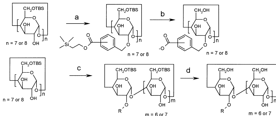
Scheme 1. Synthesis of 2- O alkylated CDs; (a) p - or m -(CH 3 ) 3 SiCH 2 CH 2 OC(O)PhCH 2 Br (or I), BaO, Ba(OH) 2 , rt 2 days; (b) TBAF, THF, 3 h Δ; (c) NaH, RCH 2 X rt, o/n R = alkyl or carboxybenzyl, (d) TBAF, THF, Δ.
